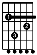
Bm7
