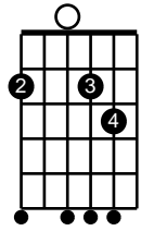
D/F#
